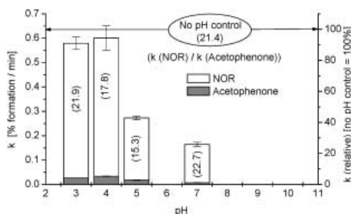
Figure 5. Plot of N -alkoxy amine (NOR) and acetophenone formation rates and their ratio as a function of pH for the reaction of TEMPO ( 2 , R=H, 1 equiv.) and ethylbenzene (10 equivs.) with t -BuOOH aq. 70% (3 equivs.)/CuCl 2 (0.1 molar) at 60 °C.
