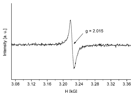
Figure 8. ESR spectrum of a solution of t -BuOOH in ethylbenzene after addition of \text{Bu}_4\text{NI} revealing the presence of t -BuOO \cdot radicals ( g = 2.015 ).
