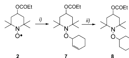
Scheme 4. Synthesis of N -alkoxy amines 7 and 8 from nitroxide 2 (R=OCOEt), cyclohexene and t -BuOOH/(cat.) Bu 4 NI followed by hydrogenation. Conditions: i) cyclohexene (10 equivs.), t -BuOOH aq. 70% (1.5 equivs.), Bu 4 NI (0.01 equivs.), 60 °C, 88% (crude); ii) hexane, 10% Pd/C (0.05 equivs.), 25 °C, H 2 (4 bar), 91% (crude).
