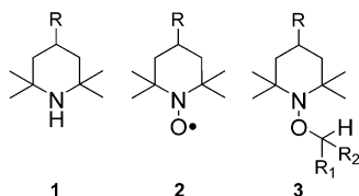
Scheme 1. N -Oxides ( 2 , nitroxides) and N -alkoxides ( 3 , NOR) of sterically hindered amines ( 1 ).
