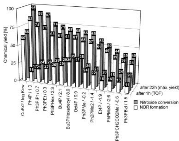
Figure 1. R 4 PI (0.01 equiv.) catalyzed reaction of 4-benzoyloxy-TEMPO ( 2 , R=OCOPh) with cyclohexane (10 equivs.) at 80 °C using aqueous 70% t -BuOOH (3 equivs.): effect of R. Results based on 3 mmol scale; log K ow = n -octanol/water partition coefficient (calculated); the reaction with Ph 4 PI as catalyst was repeated on a 35 mmol scale to afford after chromatography 63% of N -alkoxy amine 3 (R=O 2 CPh, R 1 =R 2 =pentamethylene).
