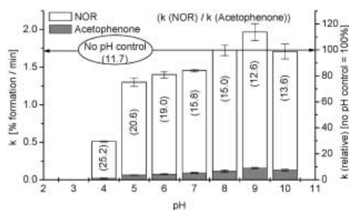
Figure 4. Plot of N -alkoxy amine (NOR) and acetophenone formation rates and their ratio as a function of pH for the reaction of TEMPO ( 2 , R=H, 1 equiv.) and ethylbenzene (10 equivs.) with t -BuOOH aq. 70% (3 equivs.)/Bu 4 NI (0.01 equiv.) at 60 °C (absence of copper).
