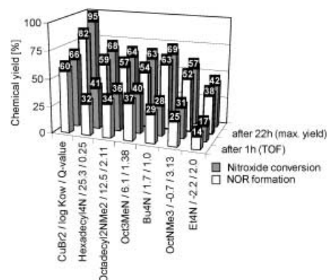
Figure 2. R 4 NI (0.01 equiv.) catalyzed reaction of 4-benzoyloxy-TEMPO ( 2 , R=OCOPh) with cyclohexane (10 equivs.) at 80 °C using aqueous 70% t -BuOOH (3 equivs): effect of R.
