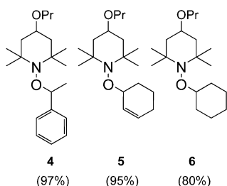
Scheme 3. Synthesis of N -alkoxy amines 4 to 6 from nitroxide 2 (R=O-propyl), hydrocarbons and t -BuOOH/(cat.) CuCl 2 . Conditions (4 mmol scale): nitroxide (1 equiv.), hydrocarbon (11.7 equivs.), t -BuOOH (53.4% in decane, 6.9 equivs.), 60 °C, CuCl 2 (1 equiv.), time ( 4 : 0.0005 equiv., 60 min; 5 : 0.0005 equiv., 12 min; 6 : 0.0019 equiv., 200 min); yields (crude) given in parenthesis.
