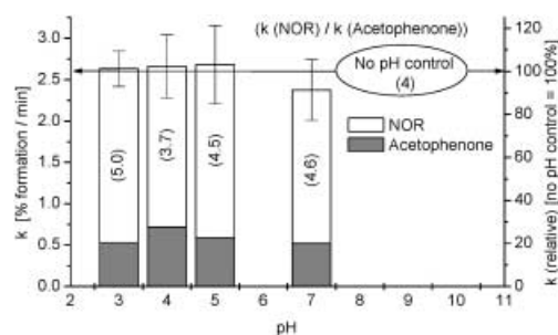
Figure 6. Plot of N -alkoxy amine (NOR) and acetophenone formation rates and their ratio as a function of pH for the reaction of TEMPO ( 2 , R=H, 1 equiv.) and ethylbenzene (10 equivs.) with t -BuOOH aq. 70% (3 equivs.)/CuCl 2 (0.1 molar) at 60 °C: effect of added phase-transfer catalyst (Oct 3 NMeCl, 0.01 equiv.).
