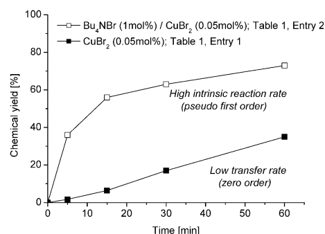
Figure 7. CuBr 2 -catalyzed reaction of TEMPO ( 2 , R=H) with ethylbenzene (10 equivs.) at 60 °C using aqueous 70% t -BuOOH (3 equivs.): effect of added phase-transfer catalyst on the N -alkoxy amine formation rate (Table 1, Entries 1 and 2).
