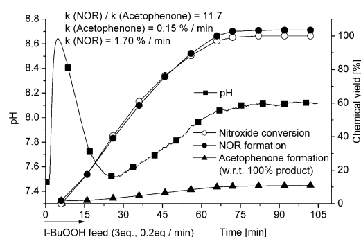
Figure 3. Overlaid plots of pH, N -alkoxy amine (NOR) formation, acetophenone formation and nitroxide conversion versus time for the reaction of TEMPO ( 2 , R=H, 1 equiv.) and ethylbenzene (10 equivs.) with t -BuOOH aq. 70% (3 equivs.)/Bu 4 NI (0.01 equivs.) at 60 °C (absence of copper). Results based on 6.4-mmol scale.
